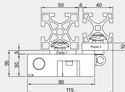
Fastening Kit A: PIL 5050 and PIL 4040
