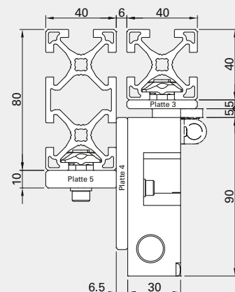
Fastening Kit B: PIL 4080 and PIL 4040
